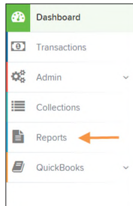
FIGURE 7 - REPORTS TAB
